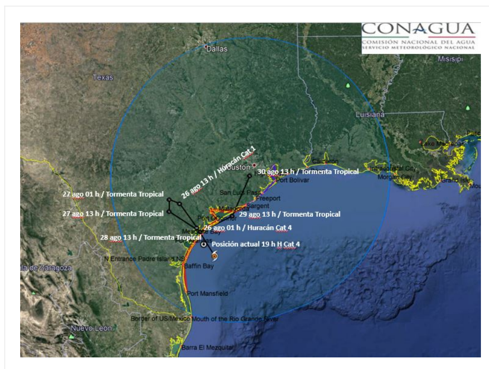
Trajectory forecast of Hurricane cat. 4 "Harvey"
